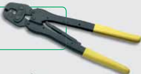
HP4-R for conductor sizes 0,25 to 1,5 sqmm
