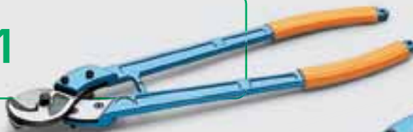
5116660500 For cutting cables 6 to 500 sqmm Weight: 3 kg Length: 800 mm
